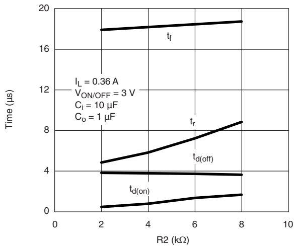
Switching Variation R2 at V_{IN} = 2.5 \text{ V} , R1 = 20 \text{ kW}
