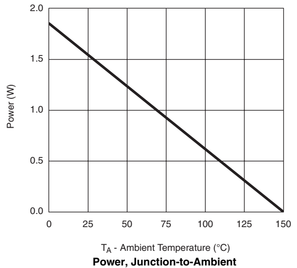
Power, Junction-to-Ambient
