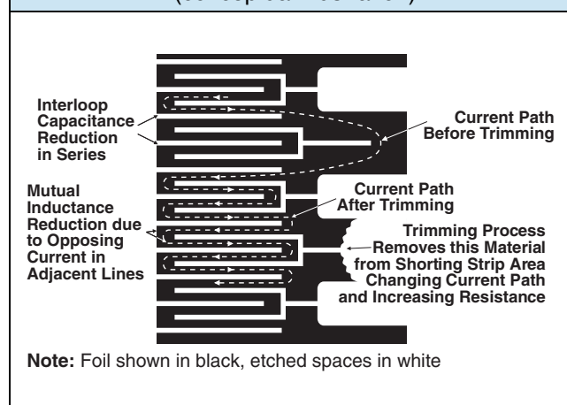
FIGURE 2 - TRIMMING TO VALUES
