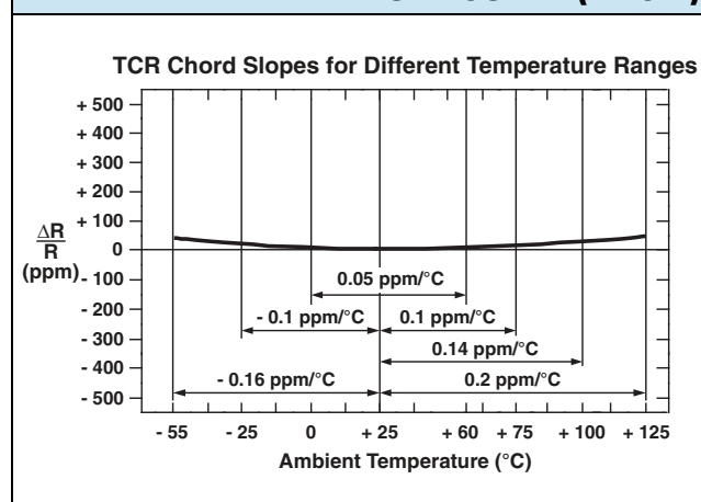
FIGURE 3 - TYPICAL RESISTANCE/TEMPERATURE CURVE (Z-FOIL)
