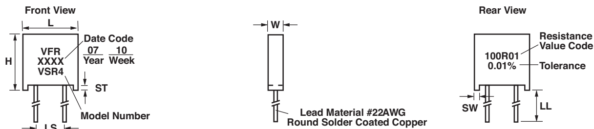
Figure 3 – Imprinting and Dimensions
