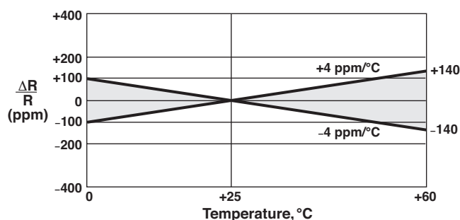
Figure 4 – Temperature Coefficient of Resistance
