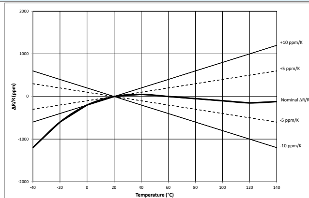
FIGURE 1 – TEMPERATURE COEFFICIENT
