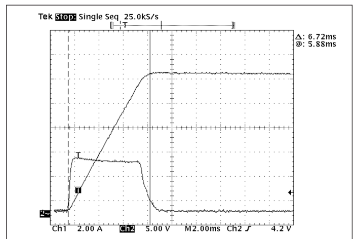
Figure 3–Inrush Limiting: Inrush current with 1000µF external capacitance.
