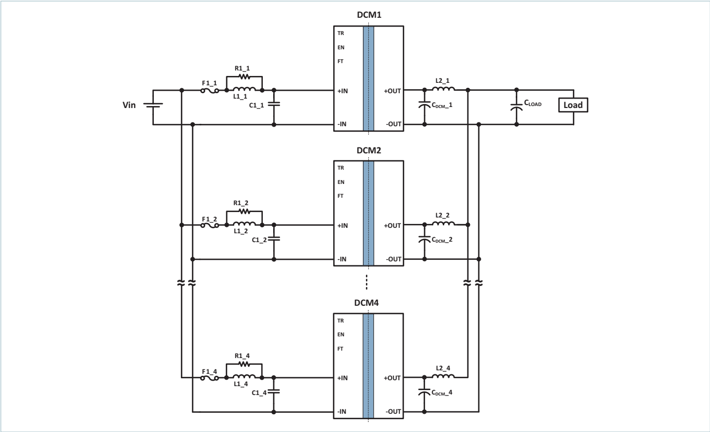
Typical Application 1: MDCM270P033M150A40 in an array of four units
