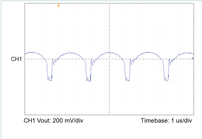
Figure 19 — Output voltage ripple, V_{IN} = 270\text{ V} , V_{OUT} = 3.3\text{ V} , C_{OUT\_EXT} = 1000\text{ }\mu\text{F} , R_{LOAD} = 0.073\text{ }\Omega
