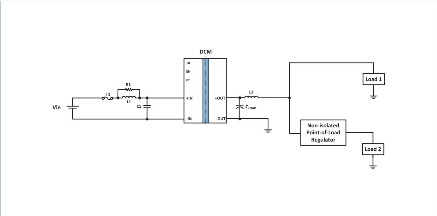
Typical Application 2: Single MDCM270P033M150A40, to a non-isolated regulator, and direct to load
