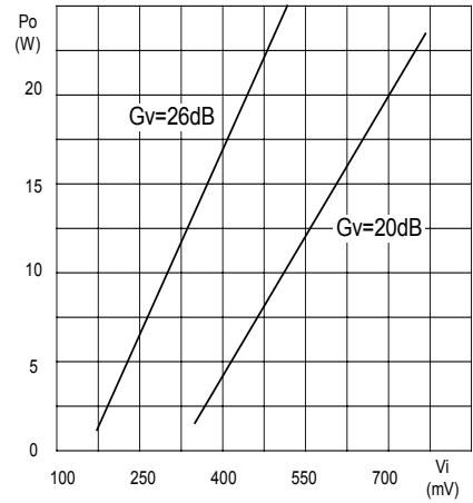
Fig. 12 Output power vs. Input level
