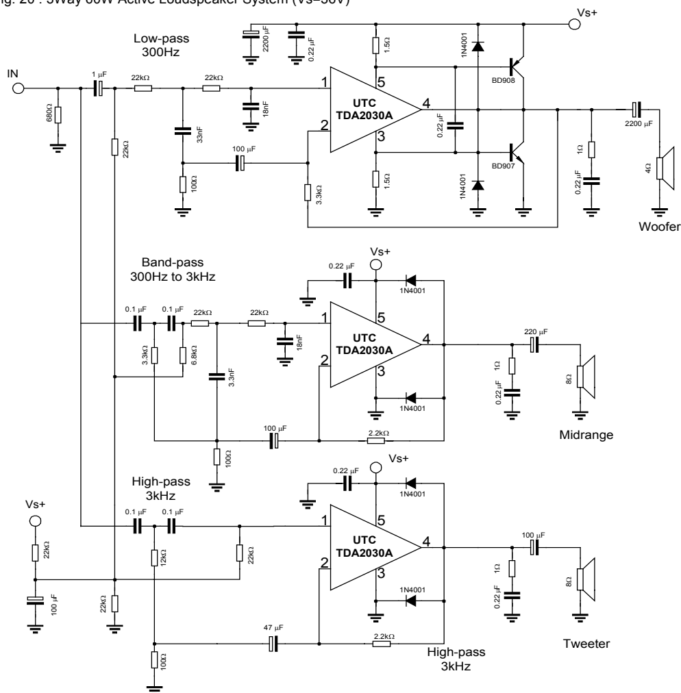
Fig. 20 : 3Way 60W Active Loudspeaker System ( V_s=36\text{V} )
