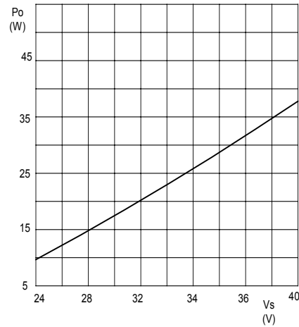
Fig. 10 Output power vs. supply voltage
