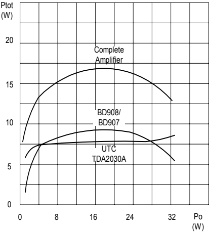
Fig. 13 Power dissipation vs. output power
