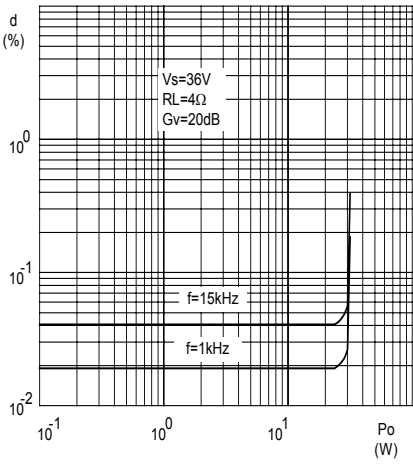
Fig. 11 Total harmonic distortion vs. output power
