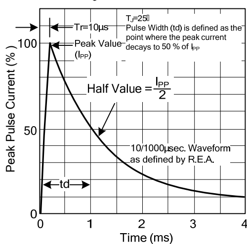
Fig 5. Pulse Waveform
