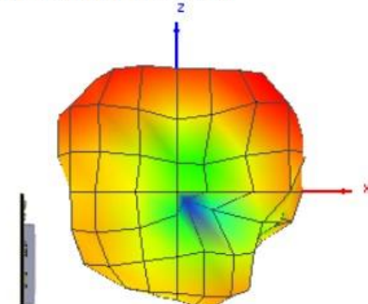
Theta = 90, Phi = 270
