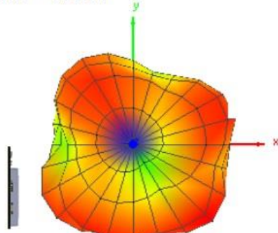
Theta = 0, Phi = 0
