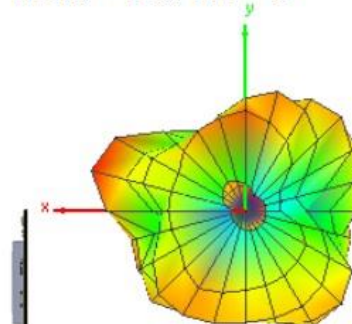
Theta = 180, Phi = 0
