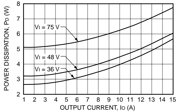
Figure 26. QHW075G1 Power Dissipation vs. Output Current at 25 °C
