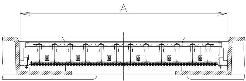
SECT. D-D (SCALE 2:1) (CONNECTOR NOT SECTION)
