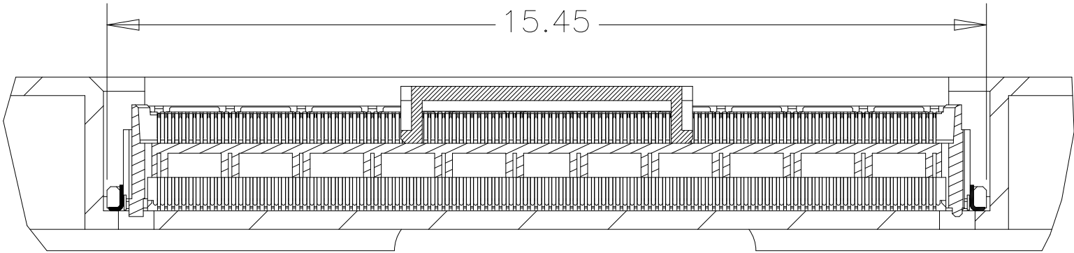
SECTION C-C SCALE 2:1
