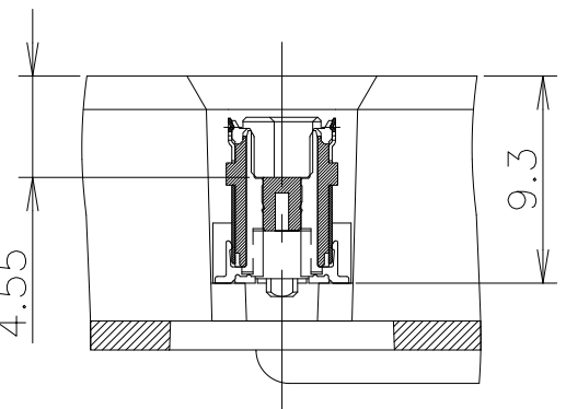
SECT. E-E (SCALE 2:1)
