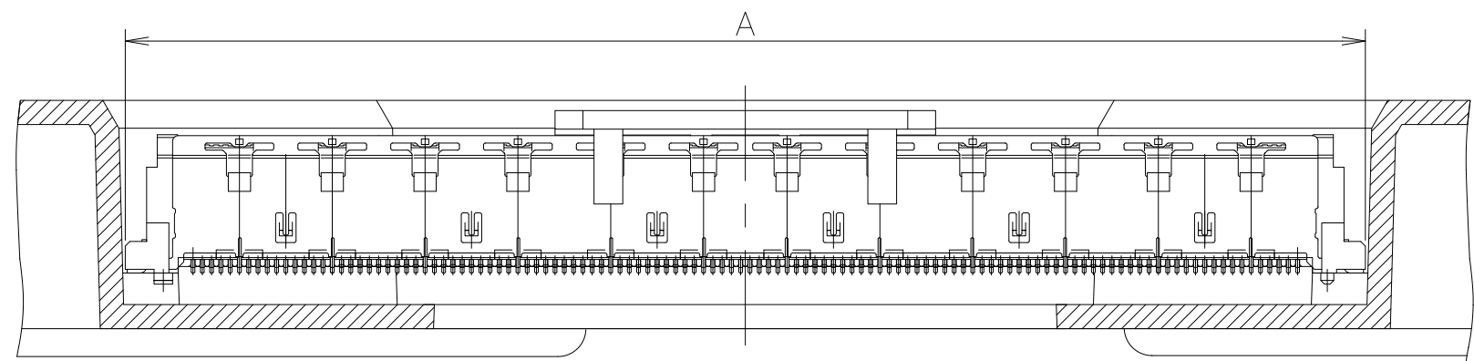
SECT. C-C (SCALE 2:1)
