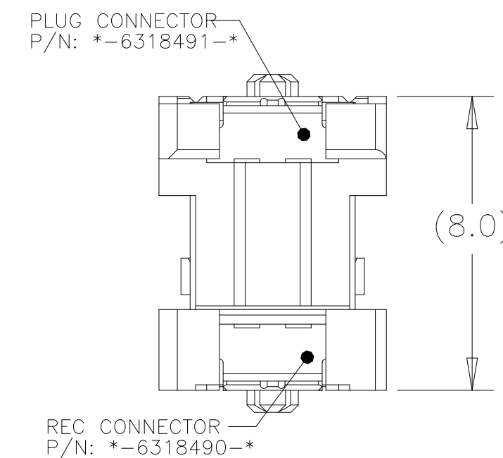
FULL-MATED CONDITION
