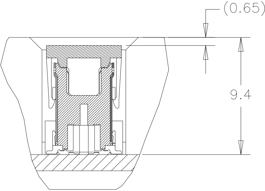
SECTION D-D SCALE 4:1
