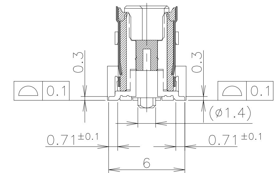
SECT. Z-Z (SIGNAL POSITION)
