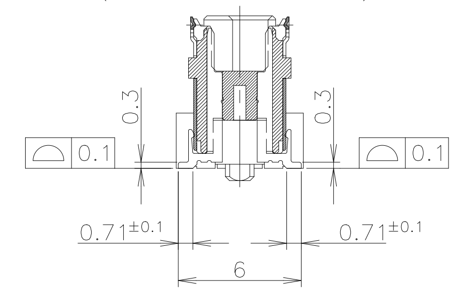
SECT. Y-Y (GROUND POSITION)
