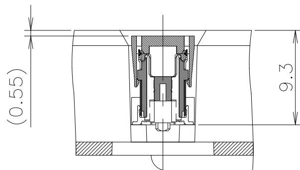
SECT. D-D (SCALE 2:1)
