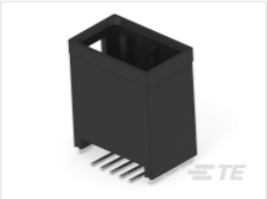
TE Part #2317525-1 2X5POS,NANOMQS,HDR ASSY, 180DEG,SMD,COD A
