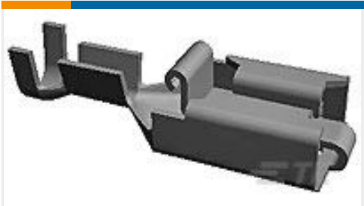
TE Model / Part #927854-6 PL 250 REC TERMINAL 17-13 AWG PTPB
