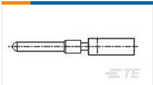
TE Model / Part #5-1437720-4 T01-CRIMP-P03
