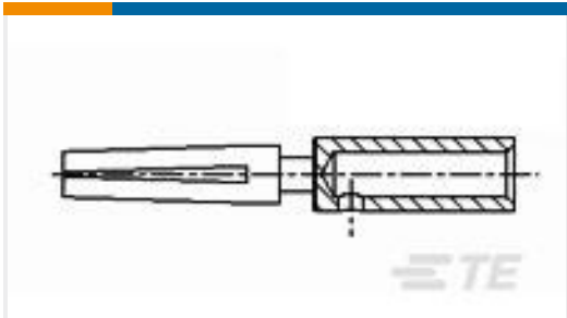
TE Model / Part #5-1437720-7 T01-CRIMP-S05=TRIAD
