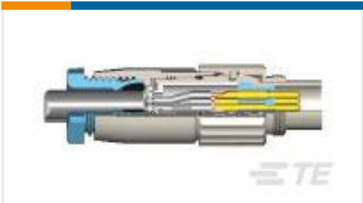
TE Model / Part #1-1437719-2 T01-0540-P05-MALE PLUG CONNECTOR-CRIMP
