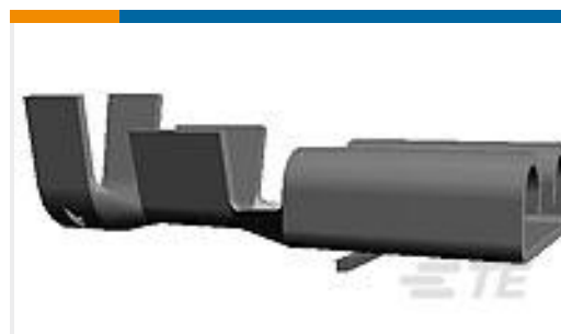
TE Part #160917-2 FF 250 REC 1-2.5MM2 TPBR
