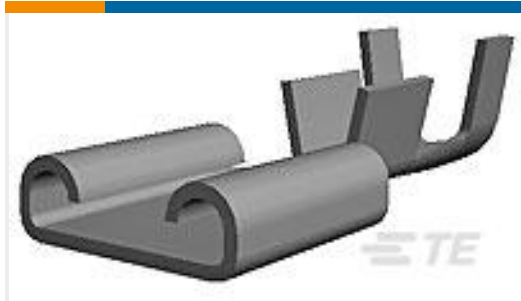
TE Part #160916-4 FASTON 250 1.0-2.5MM TPPBR
