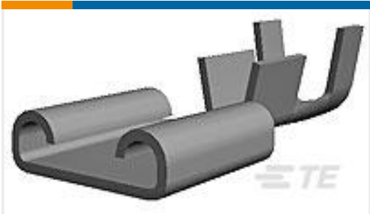
TE Part #3-160256-1 FAST 250 REC 1.0-2.5MM2 0.40X63.50 TPPB
