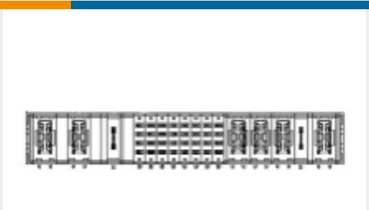
TE Part #2314577-1 R/A HEADER, MULTI- BEAM XLE, VITA 62
