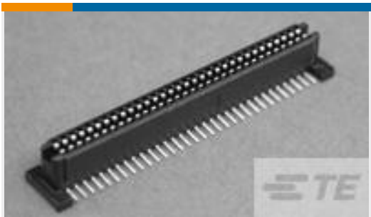
TE Part #1766501-1 ATCA ASSY, Vertical Backplane,
