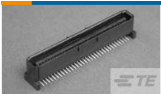
TE Part #5120526-1 1FHP,64,30A/S,S,N,S09,11,14
