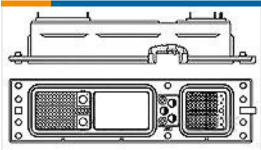
TE Part #2101650-1 A600R,Sz2,12072/ / 85 all FR
