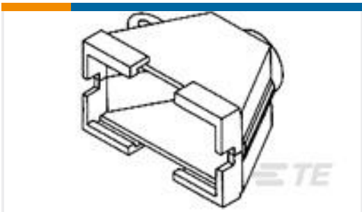
TE Part #350523-1 15P STR/REL HSG HNGD V0 RED
