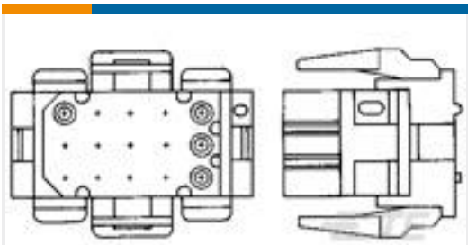
TE Part #1-640523-0 15P MR II PLUG HSG V0 RED
