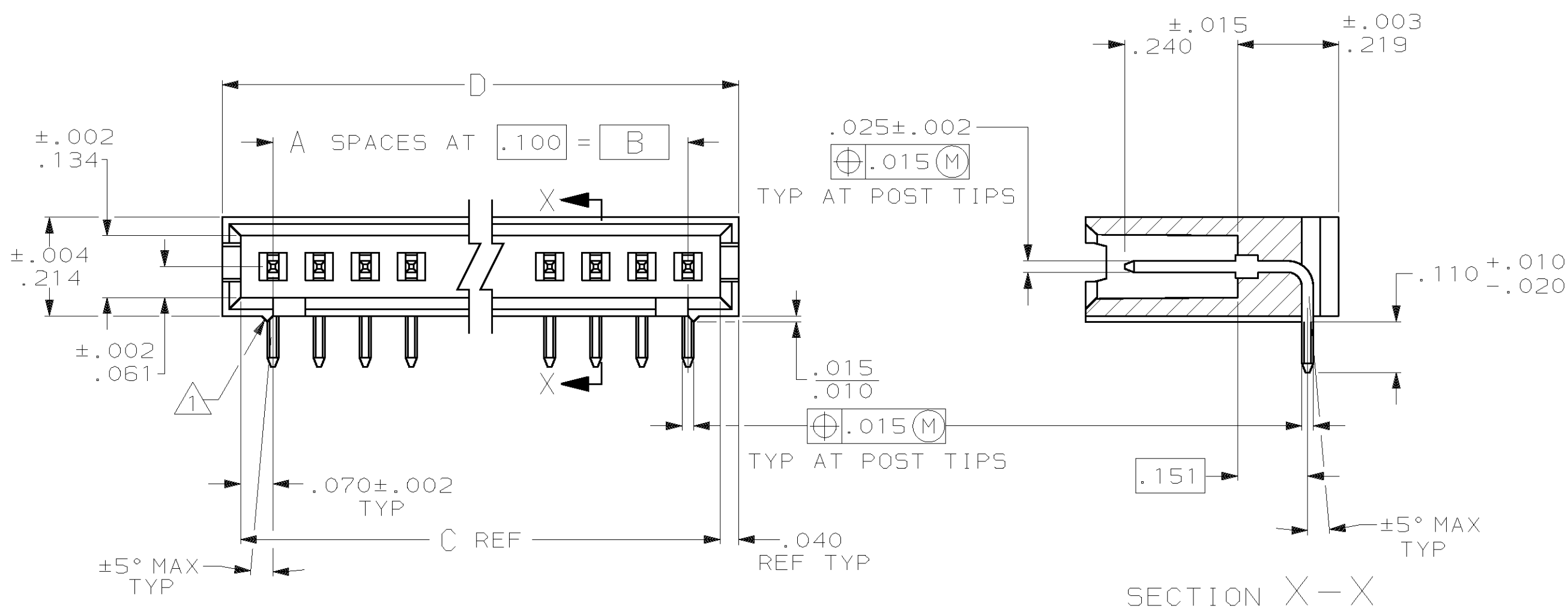
SECTION X-X
