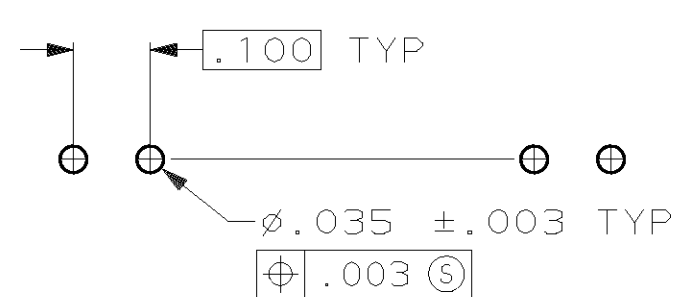
RECOMMENDED HOLE LAYOUT
