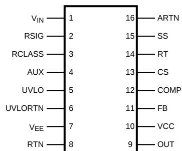
Figure 2. 16 Lead TSSOP
