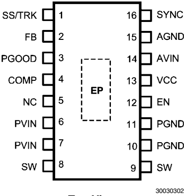
Top View eTSSOP-16 Package
