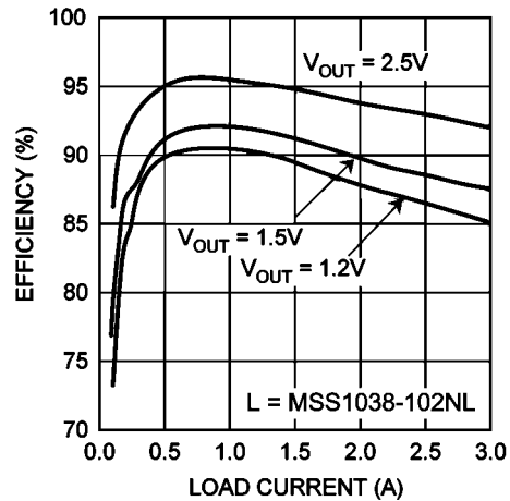
Efficiency vs. Load Current ( V_{IN} = 3.3V , f_{SW} = 1.5 MHz)
