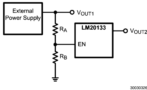
FIGURE 6. Sequencing LM20133 with Precision Enable
