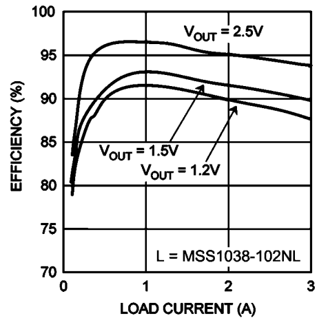
Efficiency vs. Load Current ( V_{IN} = 3.3V , f_{SW} = 500\text{ kHz} )
