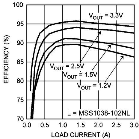
Efficiency vs. Load Current ( V_{IN} = 5V , f_{SW} = 1\text{ MHz} )
