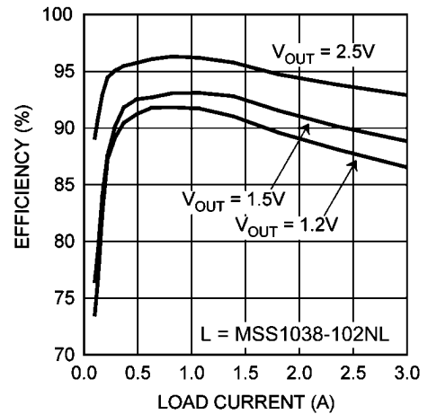
Efficiency vs. Load Current ( V_{IN} = 3.3V , f_{SW} = 1\text{ MHz} )
