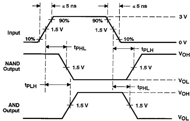
VOLTAGE WAVEFORMS
