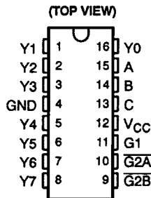
54ACT11138 ... J PACKAGE 74ACT11138 ... D, N, OR PW PACKAGE
