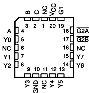
54ACT11138 ... FK PACKAGE (TOP VIEW)
