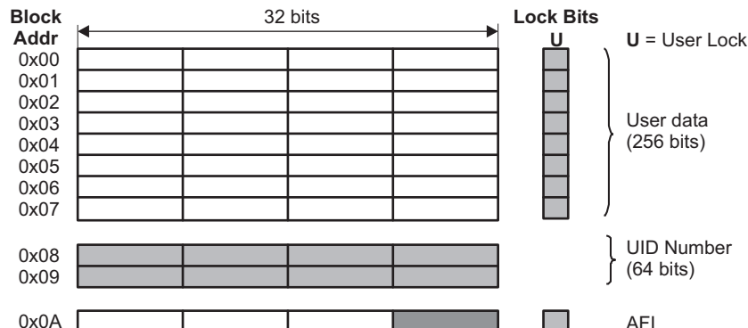
Figure 1. Memory Organization
