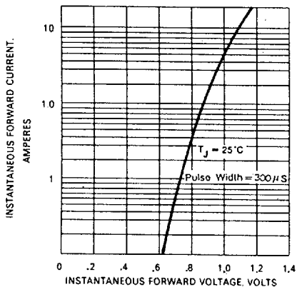
FIG.3-TYPICAL FORWARD CHARACTERISTICS
