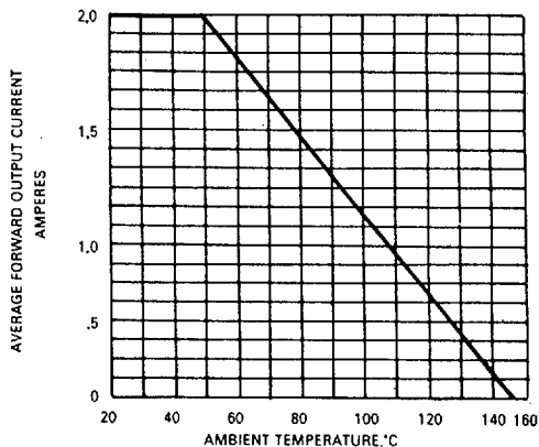
FIG.2: FORWARD DERATING CURVE OUTPUT RECTIFIED CURRENT
