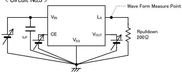
< Circuit No.3 >
