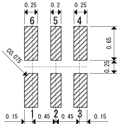
USPN-6 Reference Pattern Layout
