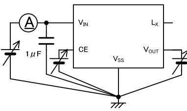
< Circuit No.2 >
