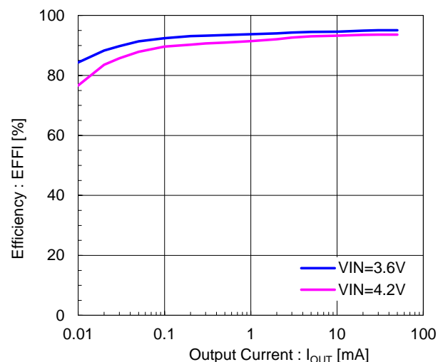
XCL210B301GR-G ( V_{OUT}=3.0\text{V} )
