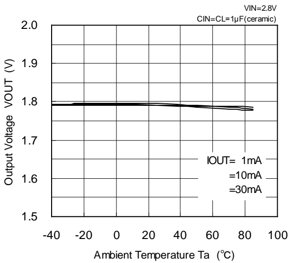
XC6202P182(1.8V)
