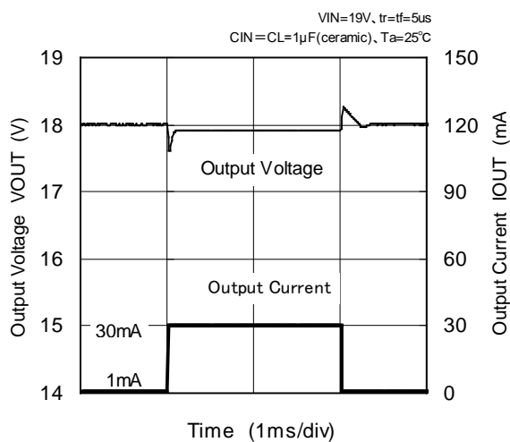
XC6202PJ02 (18V)
