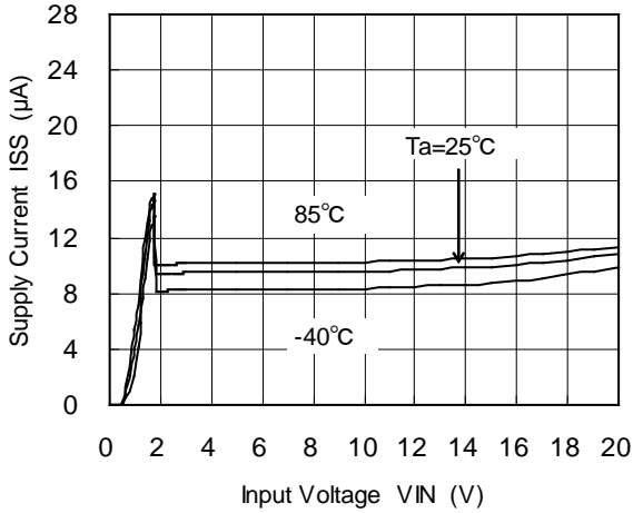
XC6202P182(1.8V)
