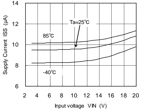
XC6202P182(1.8V)
