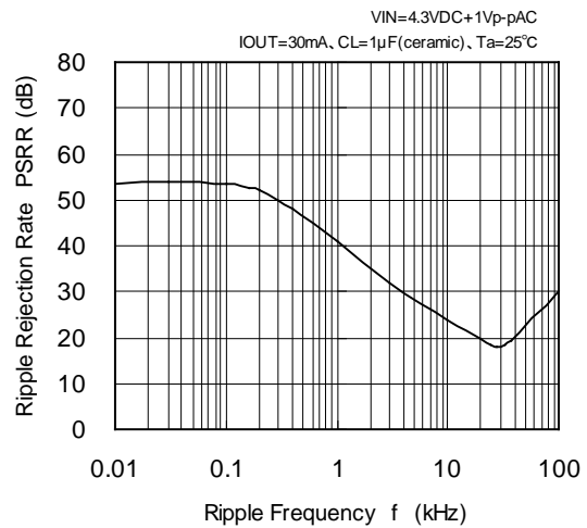
XC6202P332 (3.3V)
