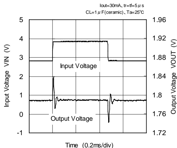
XC6202P182(1.8V)
