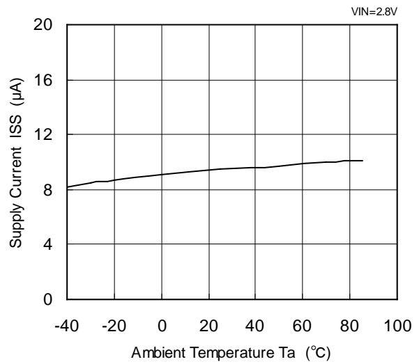
XC6202P182(1.8V)
