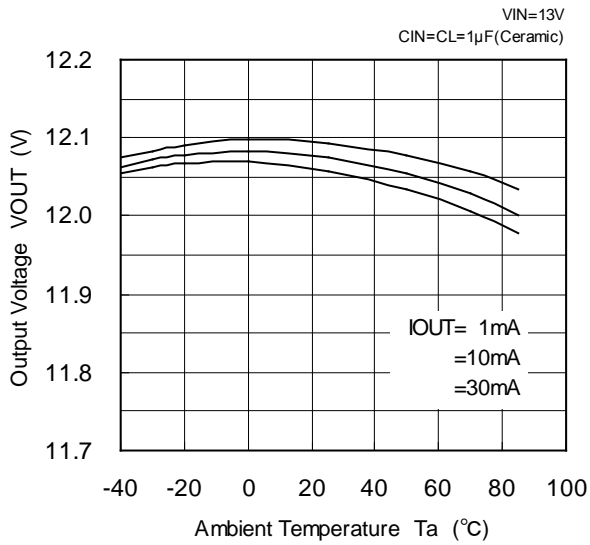
XC6202PC02(12V)
