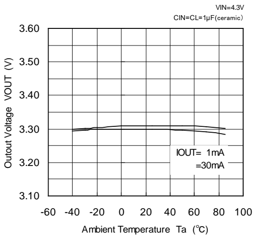
XC6202P332 (3.3V)
