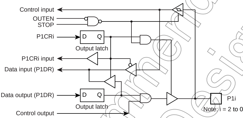
Figure 5-3 P1 Port
