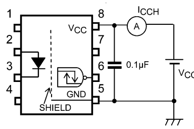
Fig. 12.1.4 ICCH Test Circuit
