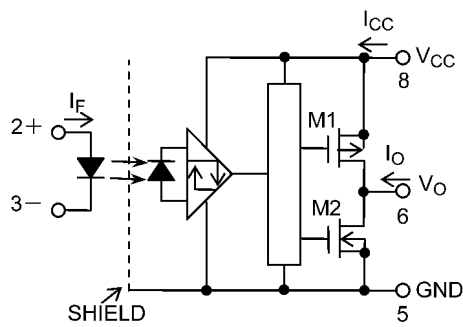
Fig. 5.1 Internal Circuit
