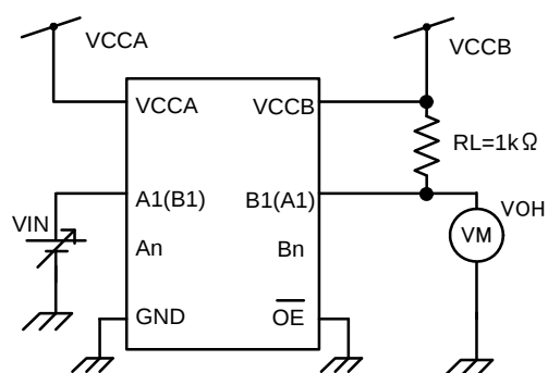
Figure 7 Test Circuit
