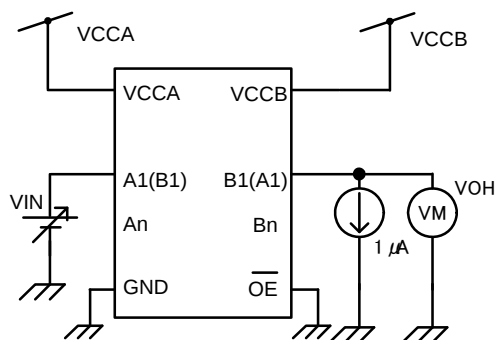
Figure 9 Test Circuit
