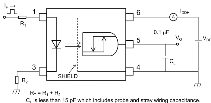
Fig. 12.1.5 Switching Time Test Circuit and Waveform
