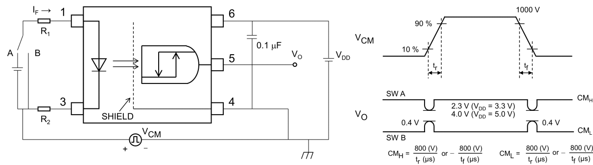
Fig. 12.1.7 Common-Mode Transient Immunity Test Circuit and Waveform
