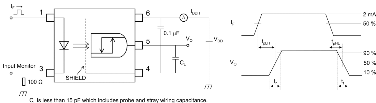
Fig. 12.1.6 Switching Time Test Circuit and Waveform
