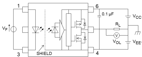
Fig. 13.1.4 V_{OL} Test Circuit
