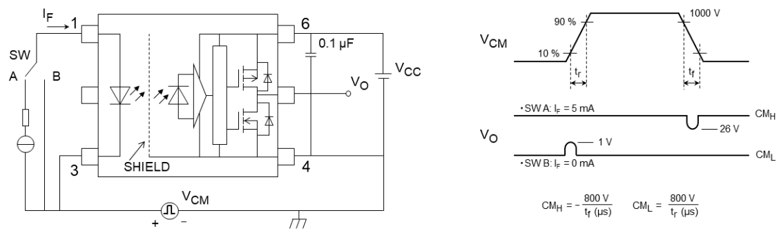
Fig. 13.1.8 Common-Mode Transient Immunity Test Circuit and Waveform
