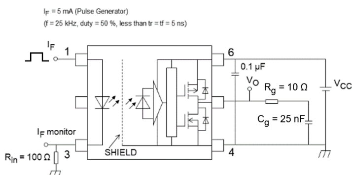
Fig. 13.1.7 Switching Time Test Circuit and Waveform
