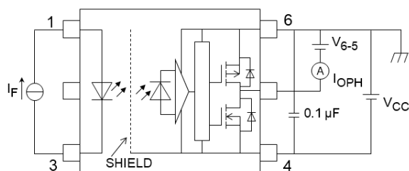
Fig. 13.1.1 I_{OPH} Test Circuit
