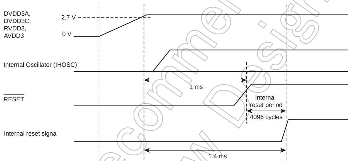
Figure 22-2 Power-on sequence
