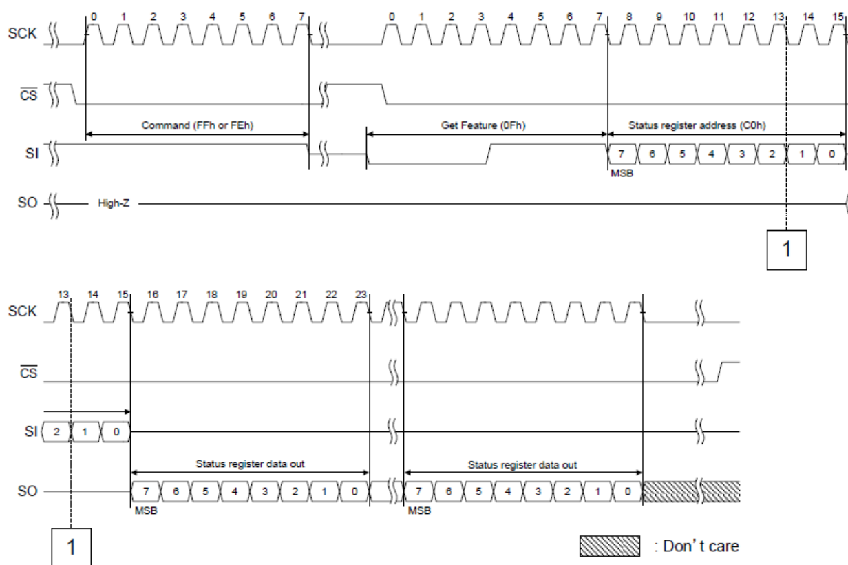
Figure 20. Reset Timing
