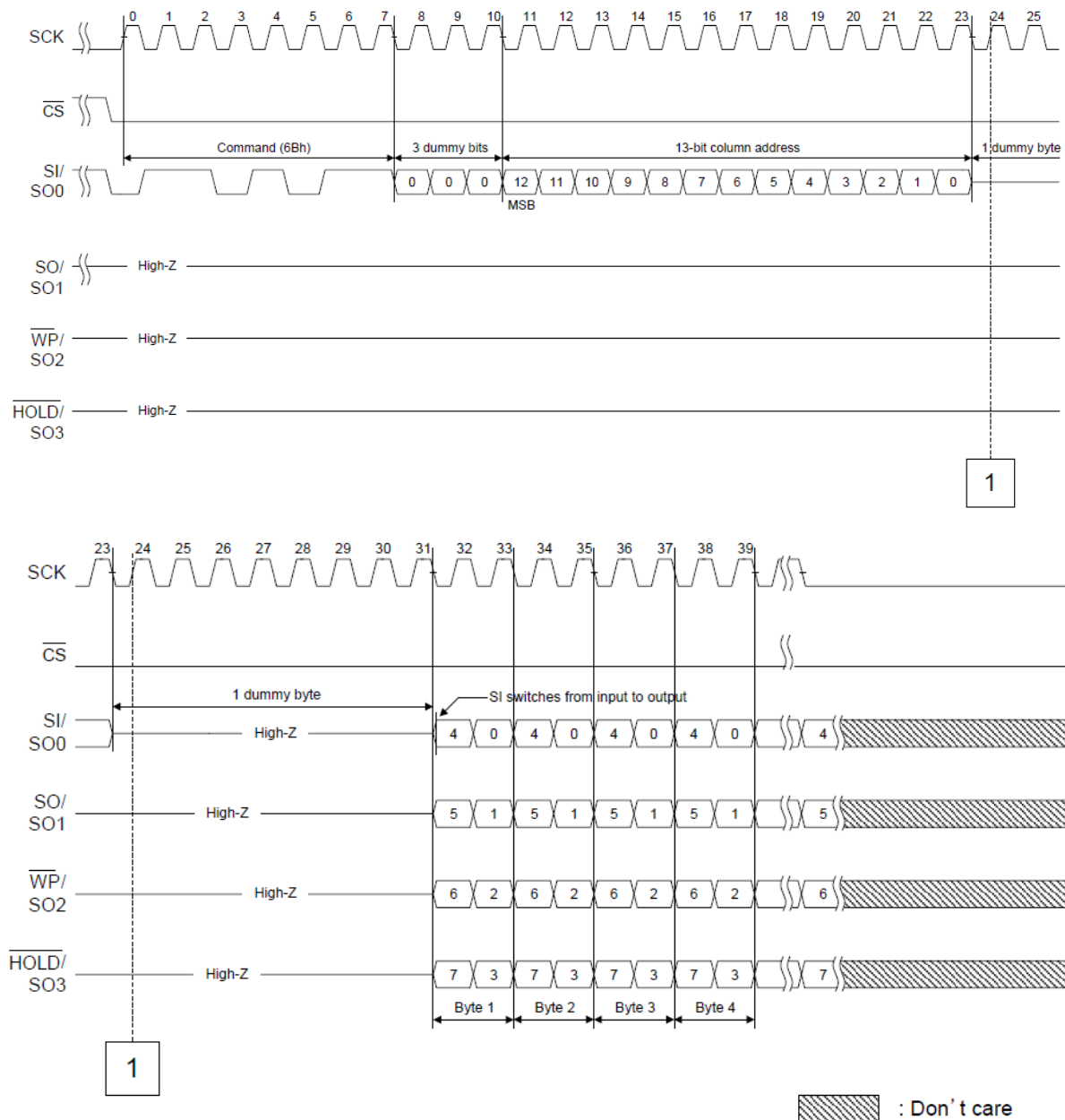
Figure 15. Page Read from Buffer x4 Timing
