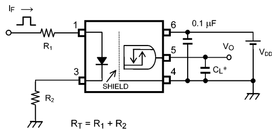
Fig. 12.1.5 Switching Time Test Circuit and Waveform
