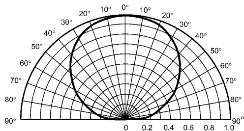
Fig. 8.7 Radiation Pattern
