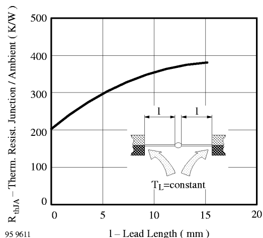
Figure 1. Thermal Resistance vs. Lead Length
