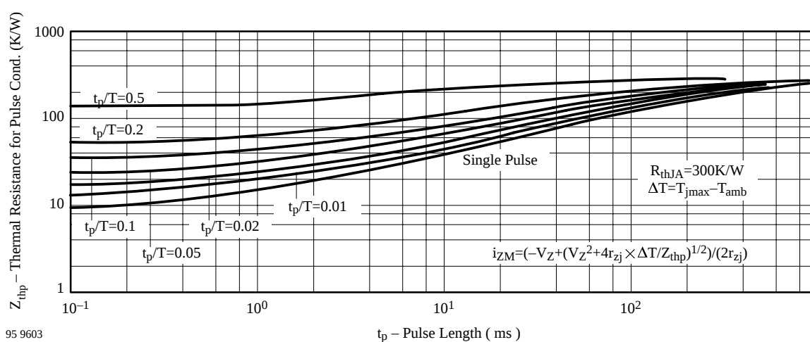
Figure 10. Thermal Response
