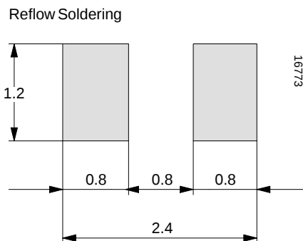
Figure 12. Recommended foot pads (in mm)
