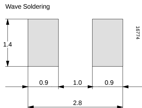
Figure 13. Recommended foot pads (in mm)
