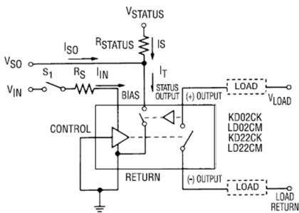
(C) 2 Terminal Input (Direct Drive) with Status
