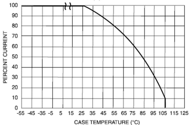
LOAD CURRENT DERATING CURVE FOR LD SERIES WITH HEAT SINK (B)
