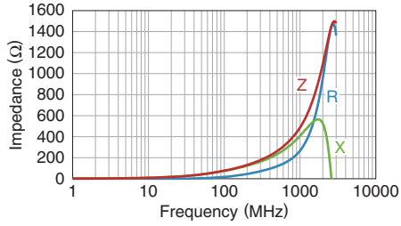
MMZ1005AFZ750V
