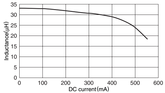
VLS3012T-330MR40
