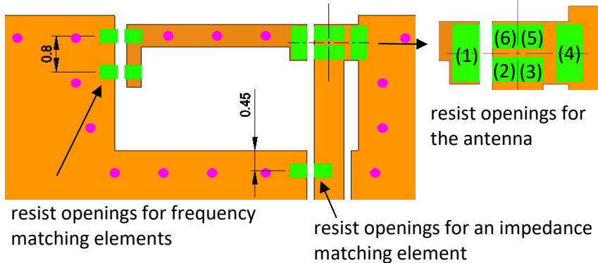
<Top Layer + resist pattern>
