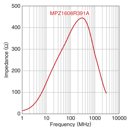
MPZ1608R type
