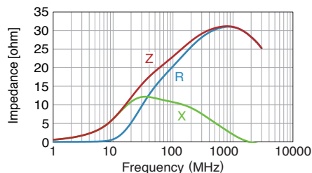
MPZ1608S600ATDH5
