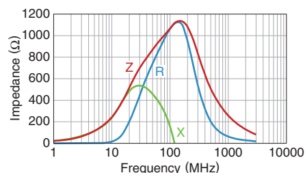
MPZ1608S102ATD25
