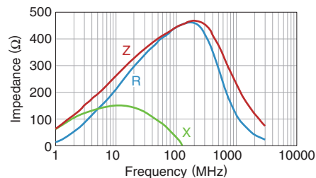
MPZ1608S300ATDH5
