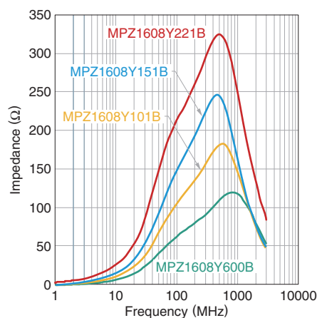
MPZ1608Y type
