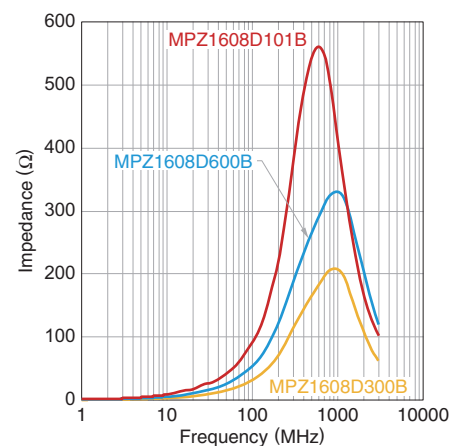
MPZ1608D type
