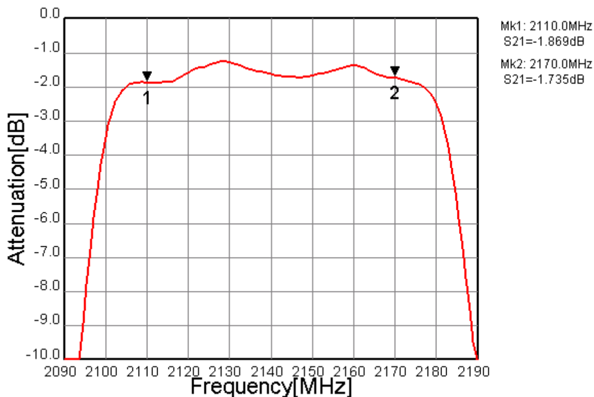
Fig.3 In-band Characteristic
