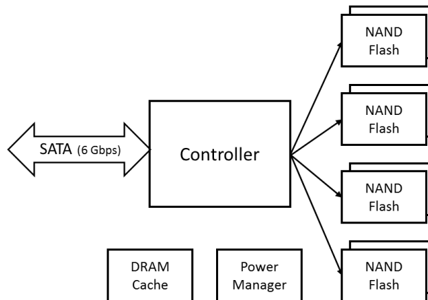
Figure 1: X-60 2.5" SATA Functional Block Diagram
