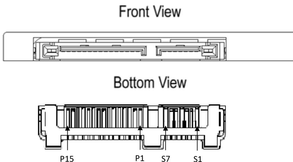
Figure 2: X-60 2.5" SATA Electrical Interface
