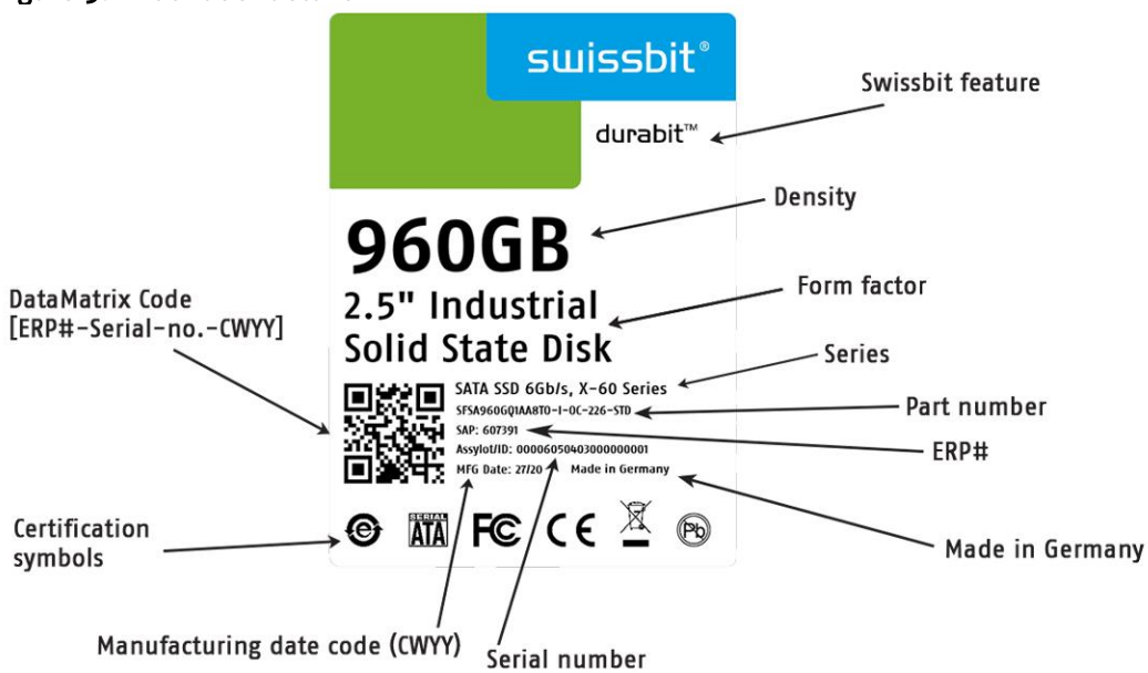
Figure 5: X-60 label details
