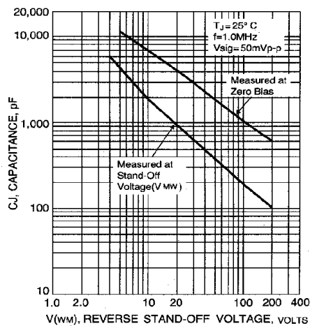
FIG. 4-TYPICAL JUNCTION CAPACITANCE
